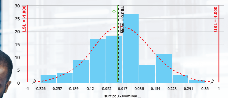
Histogram
