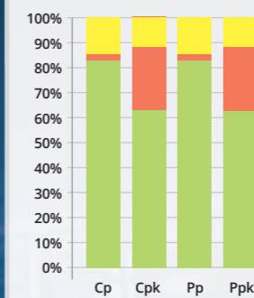
SPC stats
